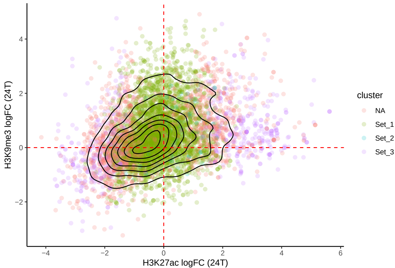
Concordance of chromatin changes at shared LTRs for 24T
